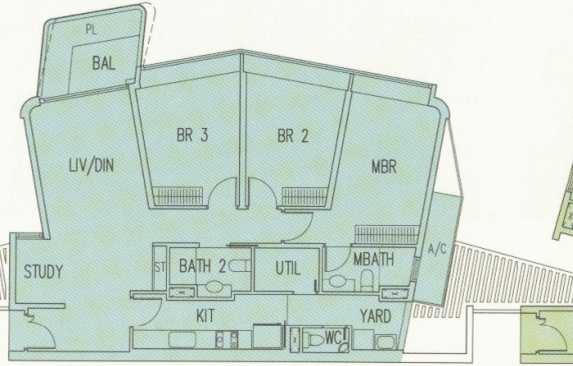
Type C3(S) #31-29 130 sqm / 1399 sqft
