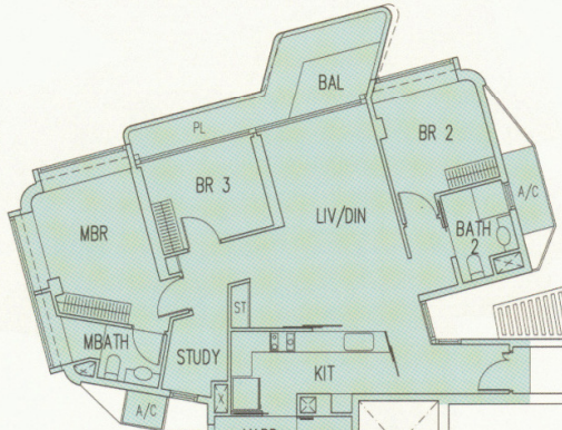
Type C3(S) #34-38 132 sqm / 1421 sqft
