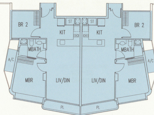
Type B1 #25-35 73 sqm / 786 sqft
