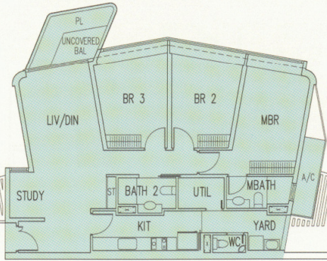
Type C3(S) #34-29 130 sqm / 1399 sqft
