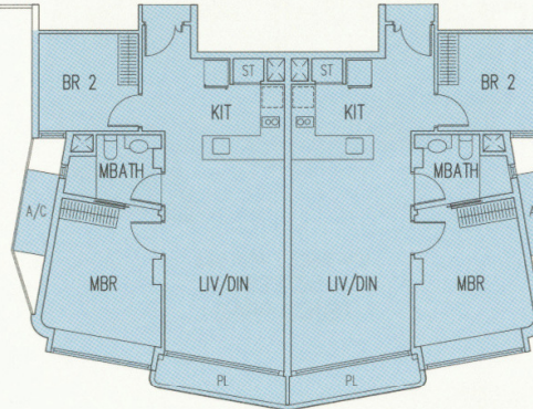
Type B1 #32-35 73 sqm / 786 sqft
